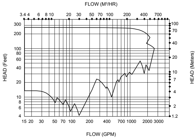
F Series Range Chart - 1750 RPM
