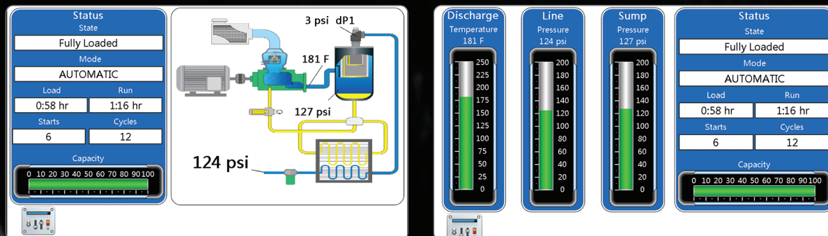
Optional Mimic Screen
